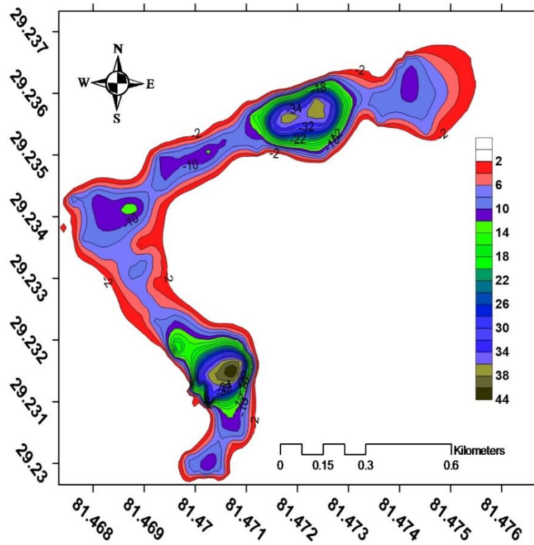
Figure 2 Bathymetry map of the Jingale Lake, one of the lakes in Ramaroshan Lake Complex
