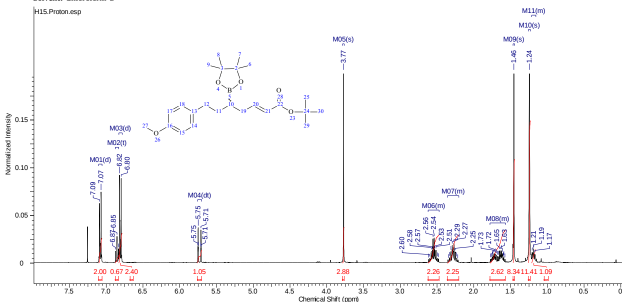
(E)-tert-butyl 7-(4-methoxyphenyl)-5-(4,4,5,5-tetramethyl-1,3,2-dioxaborolan-2-yl)hept-2-enoate (5)
