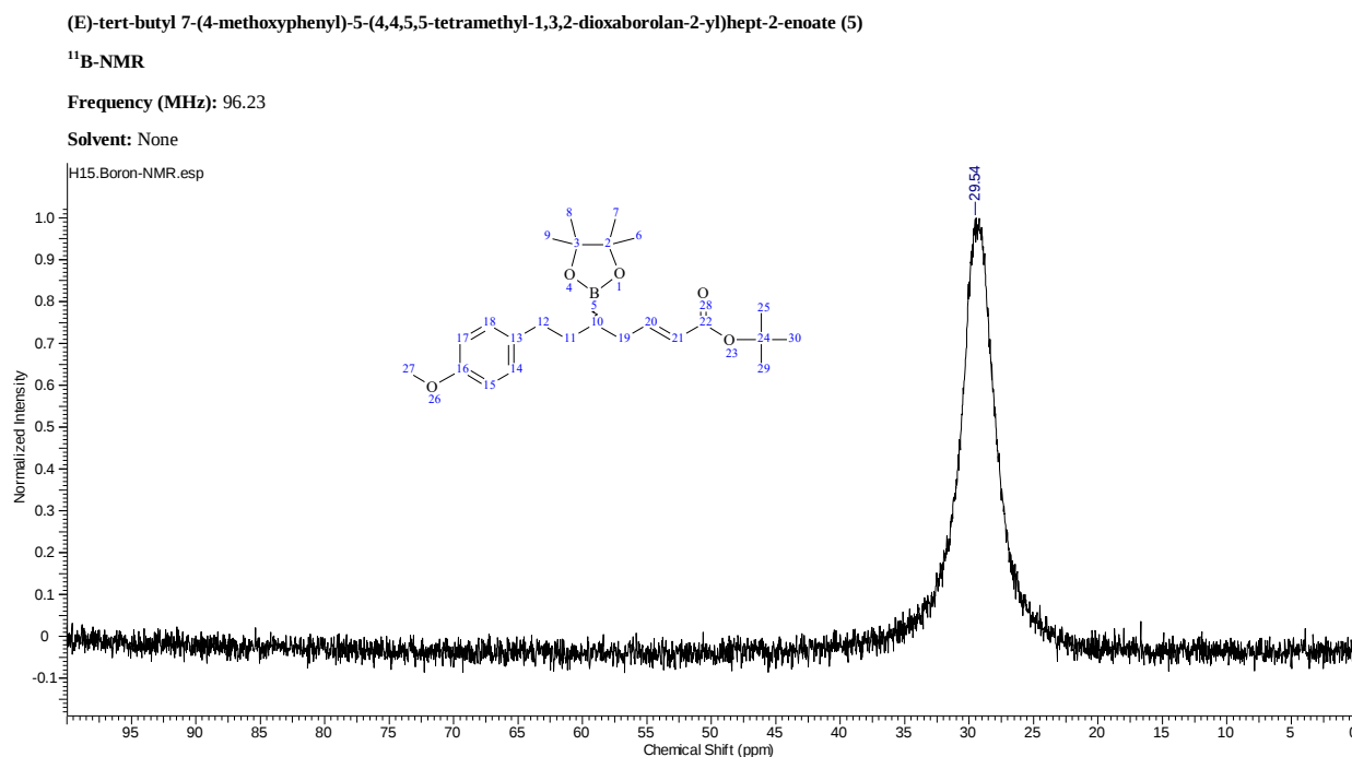
(E)-tert-butyl 7-(4-methoxyphenyl)-5-(4,4,5,5-tetramethyl-1,3,2-dioxaborolan-2-yl)hept-2-enoate (5)
