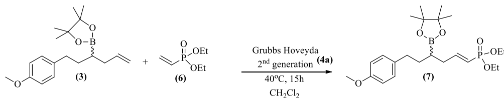
Figure 3: (E)-diethyl (6-(4-methoxyphenyl)-4-(4,4,5,5-tetramethyl-1,3,2-dioxaborolan-2-yl)hex-1-en-1-yl)phosphonate
