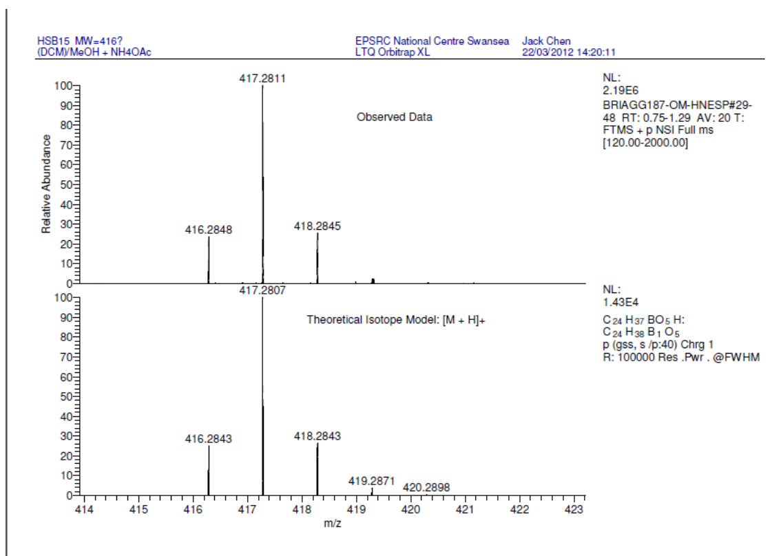
(E)-tert-butyl 7-(4-methoxyphenyl)-5-(4,4,5,5-tetramethyl-1,3,2-dioxaborolan-2-yl)hept-2-enoate (5)
