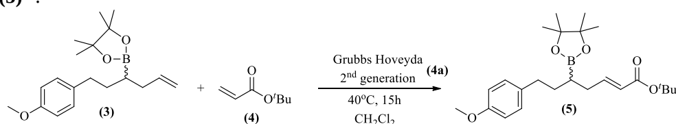
Figure 2: ( E )- tert -butyl 7-(4-methoxyphenyl)-5-(4,4,5,5-tetramethyl-1,3,2-dioxaborolan-2-yl)hept-2-enoate
