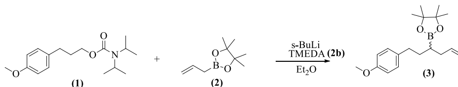
Figure 1: Synthesis of 2-(1-(4-methoxyphenyl)hex-5-en-3-yl)-4,4,5,5-tetramethyl-1,3,2-dioxaborolane
