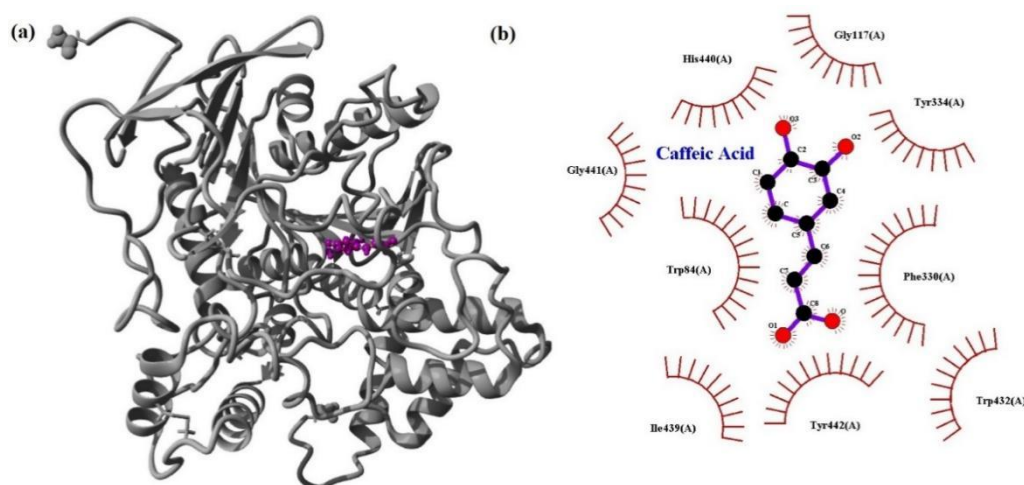
Figure 2. Molecular interactions of caffeic acid in the active site of AChE showed in the three-dimensional (caffeic acid and AChE is visualized in a purple and grey color, respectively) (a) and two-dimensional visualization (b).
