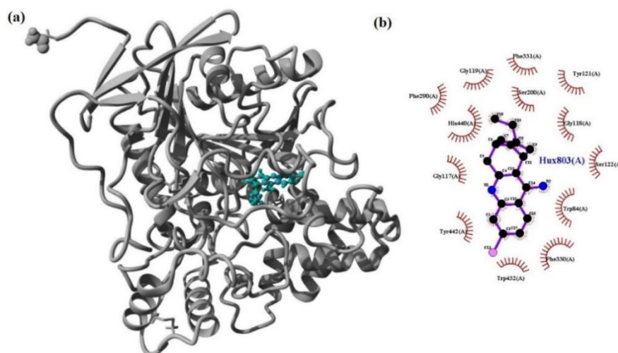
Figure 1. Molecular interactions of the native ligand i.e., huprine X in the active site of AChE showed in the three-dimensional (huprine X and AChE is visualized in a cyan and grey color, respectively) (a) and two-dimensional visualization (b).
