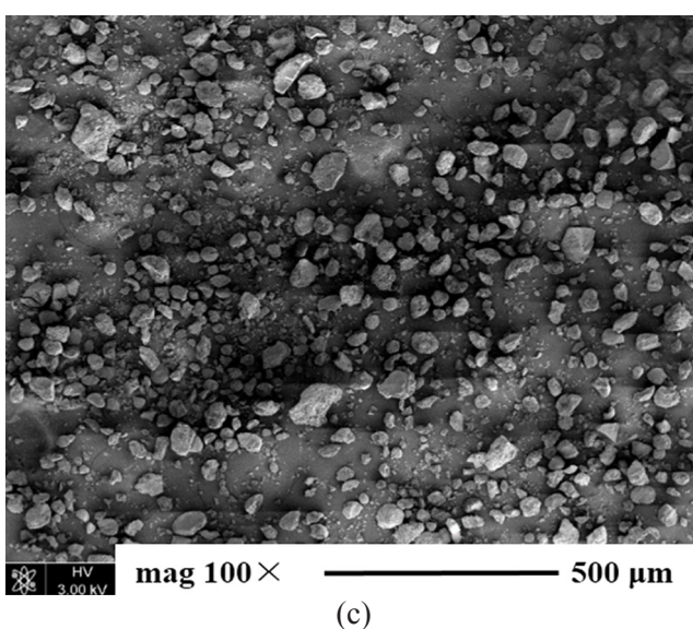
Figure 2. SEM micrographs of the (a) i-Mg/Ti/Si; (b) i-V/Ti/Si; (c) i-Mg/V/Ti/Si catalyst.
