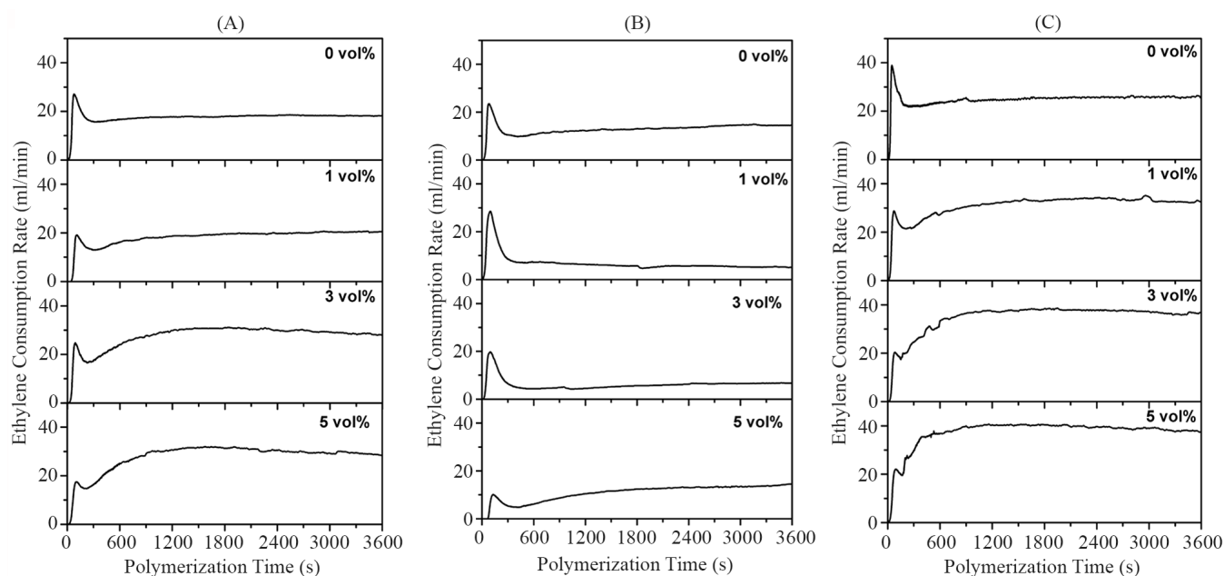
Figure 6. Kinetic curves of ethylene/1-hexene copolymerization (A) i -Mg/Ti/Si; corresponding to Run 2, 7, 8, 9; (B) i -V/Ti/Si; corresponding to Run 10, 16, 17, 18; (C) i -Mg/V/Ti/Si; corresponding to Run 21, 25, 26, 27). Conditions: catalyst 100 mg, ethylene 0.15 MPa, n -heptane 70 mL, TIBA, 1 h.
