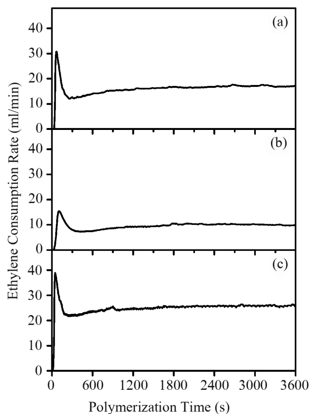
Figure 4. Kinetic curves of ethylene homopolymerization activities of different catalysts with the same Al/Ti molar ratio of 10 (corresponding to Run 3, 12, 21; (a) i-Mg/Ti/Si; (b) i-V/Ti/Si; (c) i-Mg/V/Ti/Si). Conditions: catalyst 100 mg, ethylene 0.15 MPa, n-heptane 70 mL, TIBA, 1 h.
