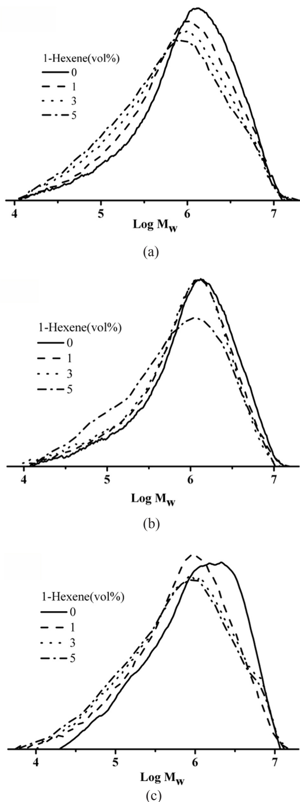
Figure 7. MWD curves of ethylene/1-hexene copolymers. (a) i-Mg/Ti/Si; (b) i-V/Ti/Si; (c) i-Mg/V/Ti/Si. Conditions: catalyst 100 mg, ethylene 0.15 MPa, n-heptane 70 mL, TIBA, 1 h.
