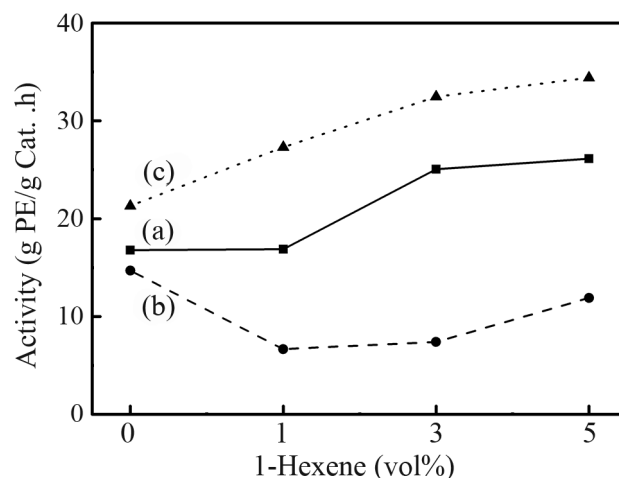
Figure 5. Ethylene/1-hexene copolymerization activities of different catalysts with different dosages of 1-hexene. (a) i-Mg/Ti/Si; (b) i-V/Ti/Si; (c) i-Mg/V/Ti/Si. Conditions: catalyst 100 mg, ethylene 0.15 MPa, n-heptane 70 mL, TIBA, 1 h.
