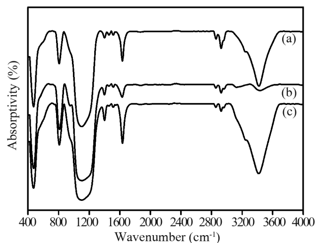
Figure 1. IR spectra of different catalysts. (a) i -Mg/Ti/Si, (b) i -V/Ti/Si, (c) Mg/V/Ti/Si catalyst.
