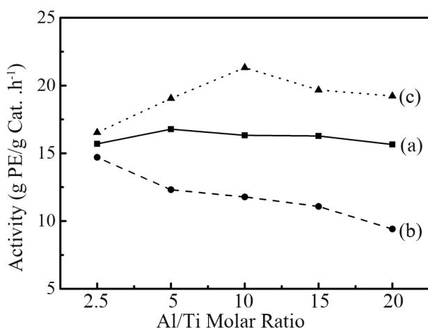
Figure 3. Ethylene homopolymerization activities of different catalysts with different Al/Ti molar ratio. (a) i-Mg/Ti/Si; (b) i-V/Ti/Si; (c) i-Mg/V/Ti/Si. Conditions: catalyst 100 mg, ethylene 0.15 MPa, n-heptane 70 mL, TIBA, 1 h.
