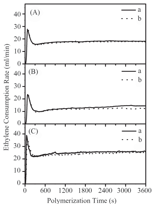
Figure 8. Kinetic curves of ethylene homopolymerization with/without hydrogen. (A): i-Mg/Ti/Si, Al/Ti=5, (a) without H 2 , (b) with H 2 , corresponding to Run 2, 6; (B): i-V/Ti/Si, Al/Ti=2.5, (a) without H 2 , (b) with H 2 , corresponding to Run 10, 15; (C): i-Mg/V/Ti/Si, Al/Ti=10, (a) without H 2 , (b) with H 2 , corresponding to Run 21, 24. Conditions: catalyst 100 mg, ethylene 0.15 MPa, n-heptane 70 mL, TIBA, 1 h, H 2 10 mL.
