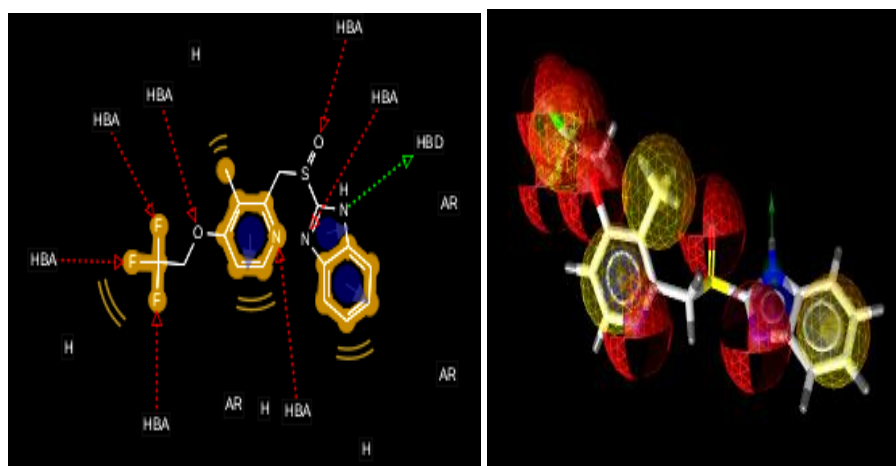
Figure 3: Pharmacophore model of Dexlansoprazole (a) 2D model (b) 3D model
