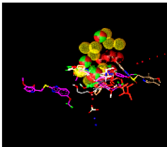
Figure 16: Pharmacophore model of all compounds
