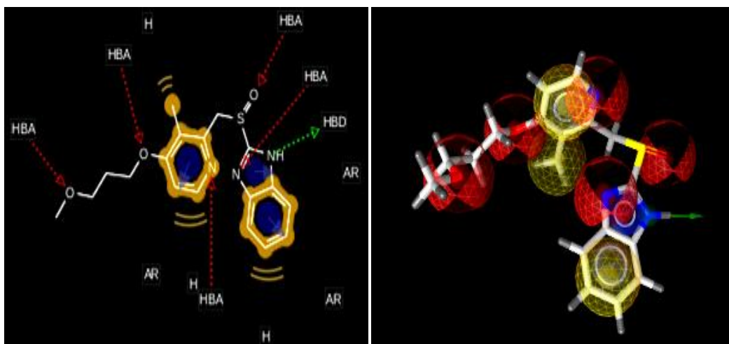
Figure 11: Pharmacophore model of Rabeprazole (a) 2D model (b) 3D model
