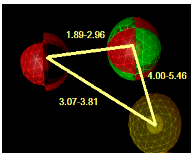
Figure 17: Distance ranges of common Pharmacophoric Features. Red sphere represents HBA, green sphere represents HBD and yellow sphere represents hydrophobic domain
