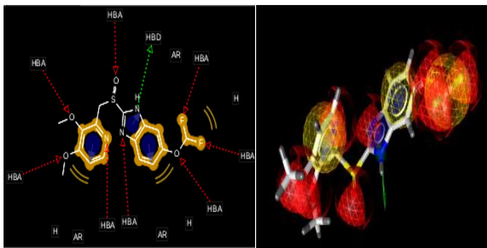
Figure 8: Pharmacophore model of Pantoprazole (a) 2D model (b) 3D model
