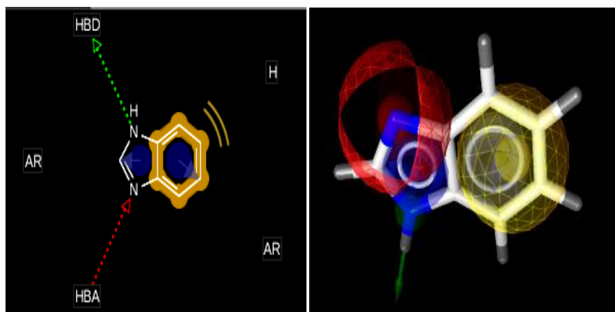
Figure 2: Pharmacophore model of Benzimidazole (a) 2D model (b) 3D model
