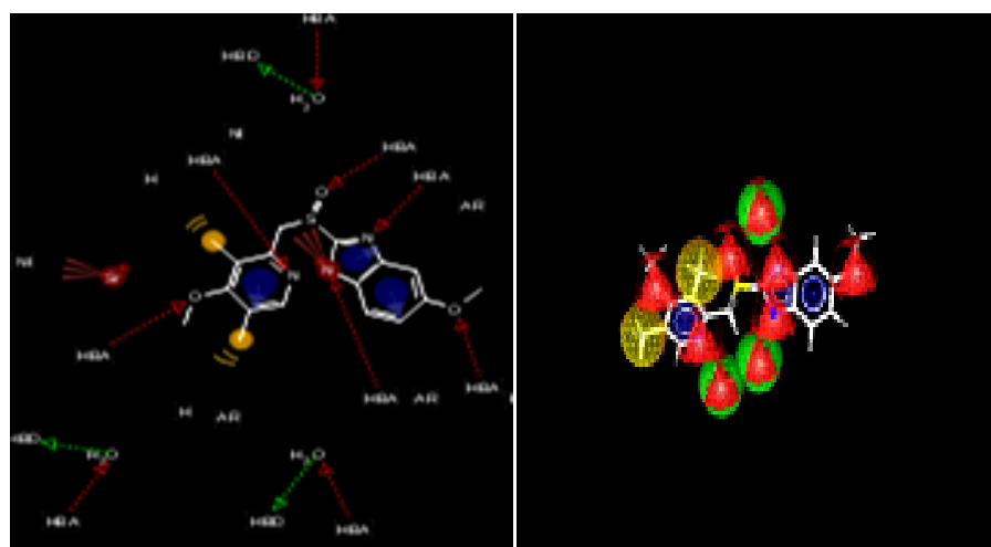
Figure 4: Pharmacophore model of Esomeprazole (a) 2D model (b) 3D model
