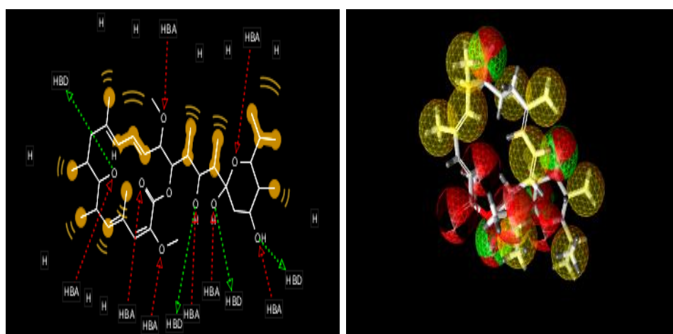
Figure 1: Pharmacophore model of bafilomycin A1 (a) 2D model (b) 3D model
