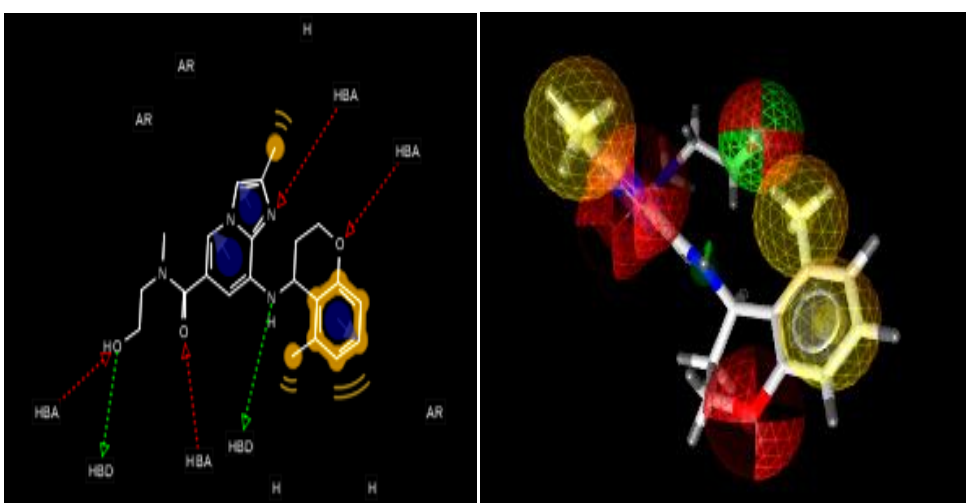
Figure 9: Pharmacophore model of PF 3716556 (a) 2D model (b) 3D model
