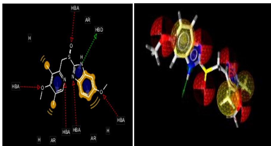
Figure 7: Pharmacophore model of Omeprazole (a) 2D model (b) 3D model
