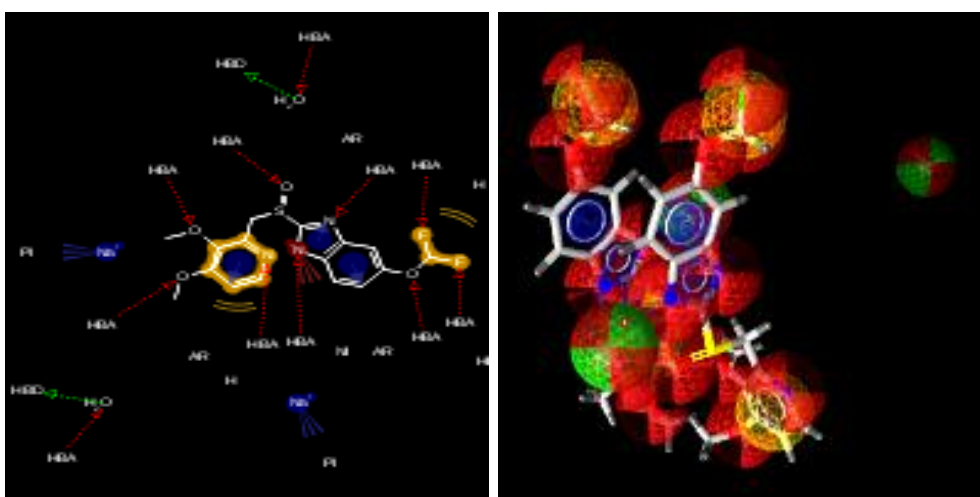
Figure 10: Pharmacophore model of Protonix (TN) (a) 2D model (b) 3D model
