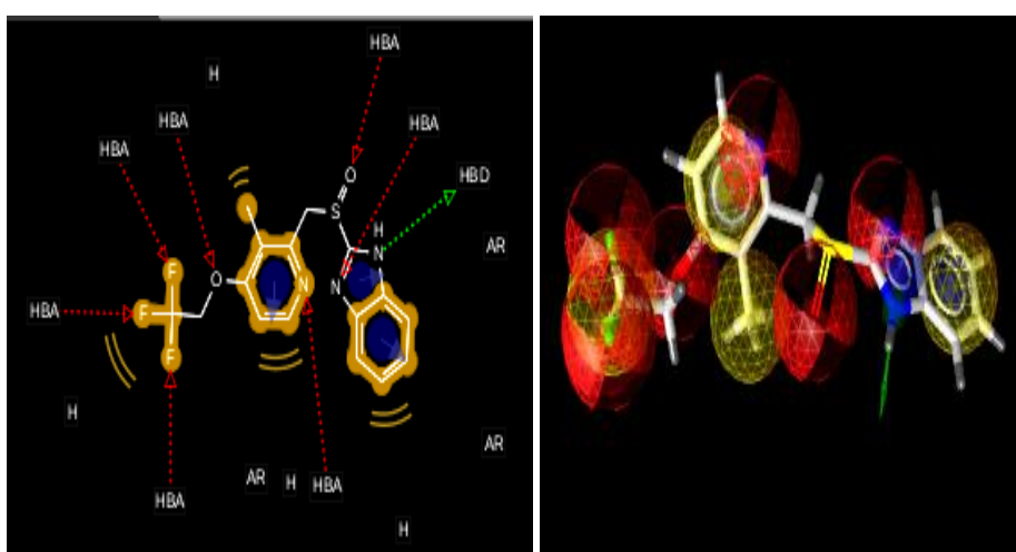
Figure 6: Pharmacophore model of Lansoprazole (a) 2D model (b) 3D model
