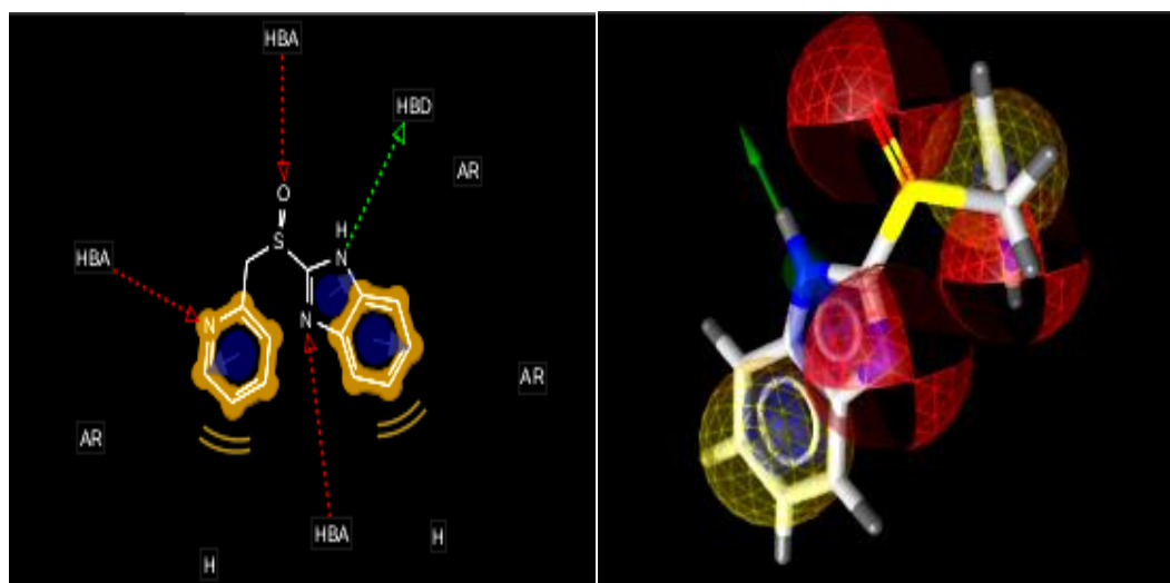
Figure 14: Pharmacophore model of Timoprazole (a) 2D model (b) 3D model
