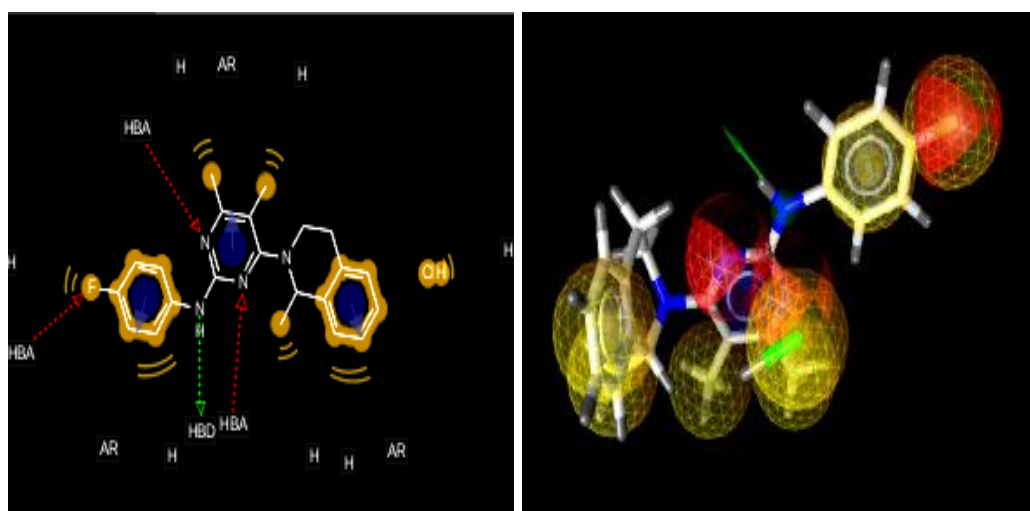
Figure 12: Pharmacophore model of Revaprazan (a) 2D model (b) 3D model
