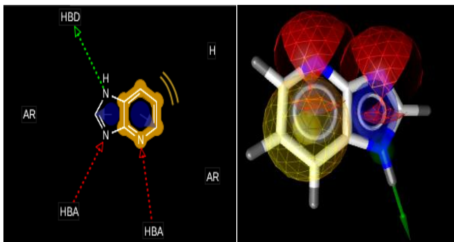
Figure 5: Pharmacophore model of imidazopyridine (a) 2D model (b) 3D model
