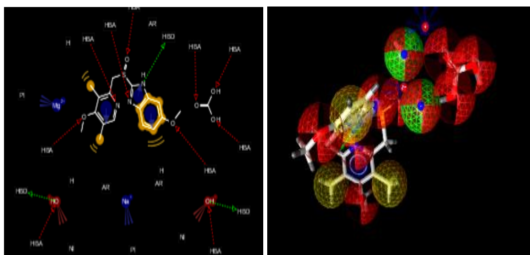
Figure 15: Pharmacophore model of Zegerid (a) 2D model (b) 3D model
