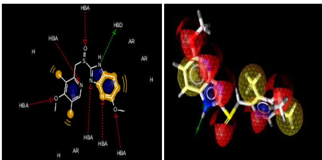
Figure 13: Pharmacophore model of Tenatoprazole (a) 2D model (b) 3D model
