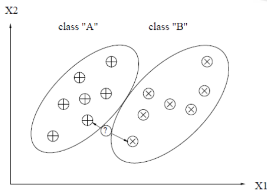
Figure 6: Correlated Features
