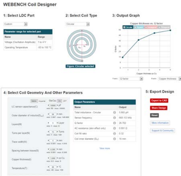
Fig. 1. WEBENCH overview showing the main components (and steps) of this tool: 1. Select LDC Part, 2. Select Coil Type, 3. Output Graph, 4. Select Coil Geometry and Other Parameters, 5. Export Design.
