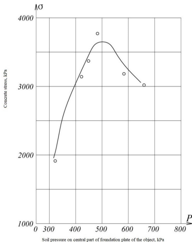
Figure 6. Object No. 6. Dependence of tensile stresses in the concrete of the upper zone of the lower plate of the box-shaped foundation on the value of the reaction pressure on the central part of the bottom.
