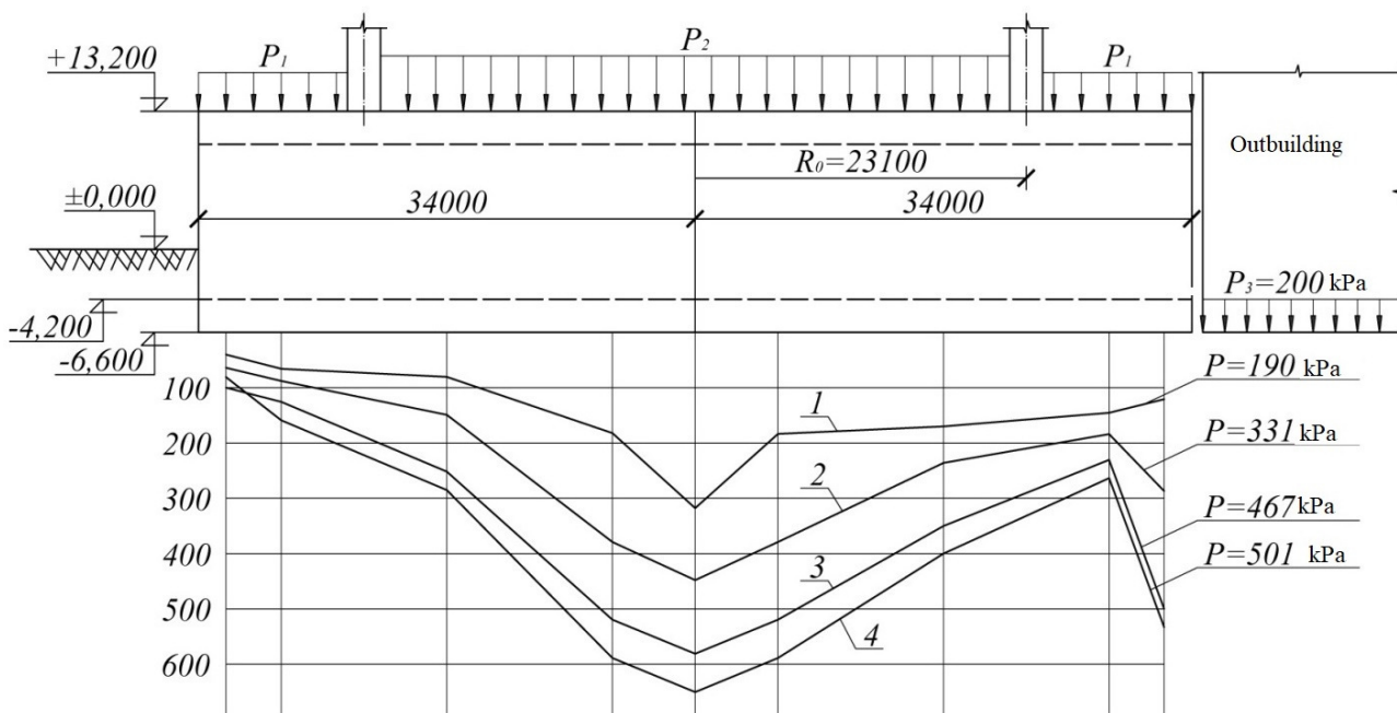
Figure 7. Facility No. 6. Deflections of the bottom plate of the box-shaped foundation at different mean pressures P_{limt} :
