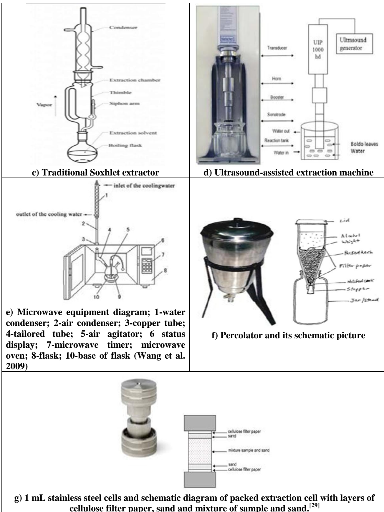
Figure 1: (a-g) Drying and extraction equipment. Figure shows an example of drying and extraction equipment discussed. Different model may be present in the market.
