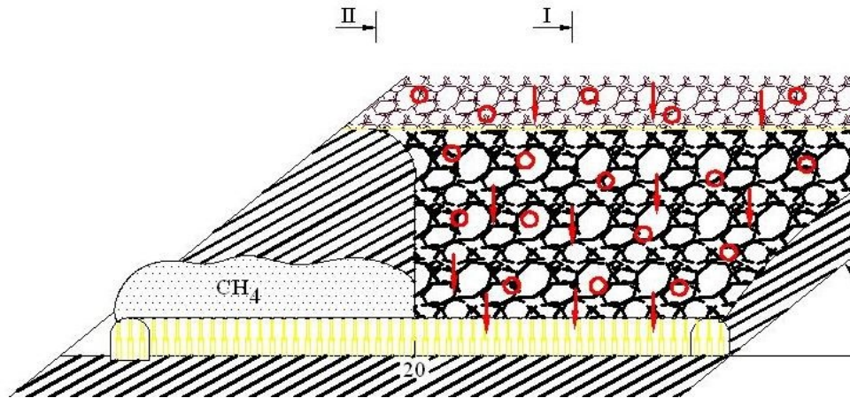
Fig. 4. Cross section through the goaf no.431, slice IV.
